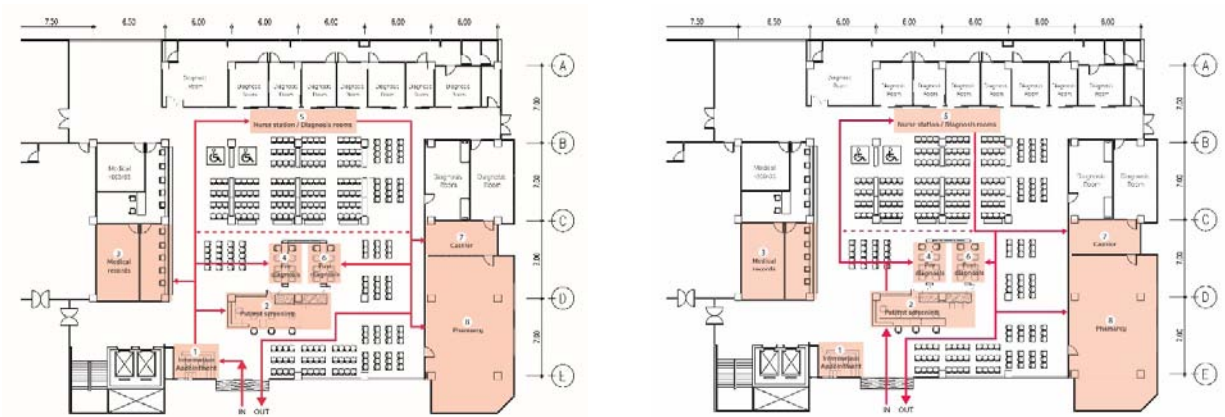
Figure 8. (Left) Layout showing circulation and workflow proposed by the design team (Right) Circulation and workflow have been adapted by users according to their familiarity.
